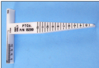
T-Handle Taper & Scale Gage #15299
