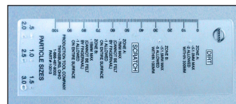
Dirt & Paint Gage #10013
