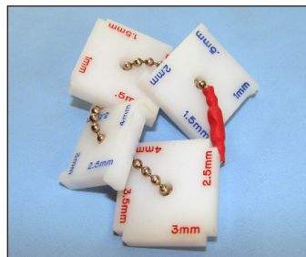
4 pcs. Gap & Flush Square Gages #15122
